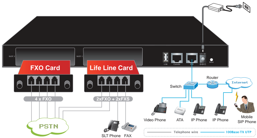
Physical Connection Topology of the IPX-2100
