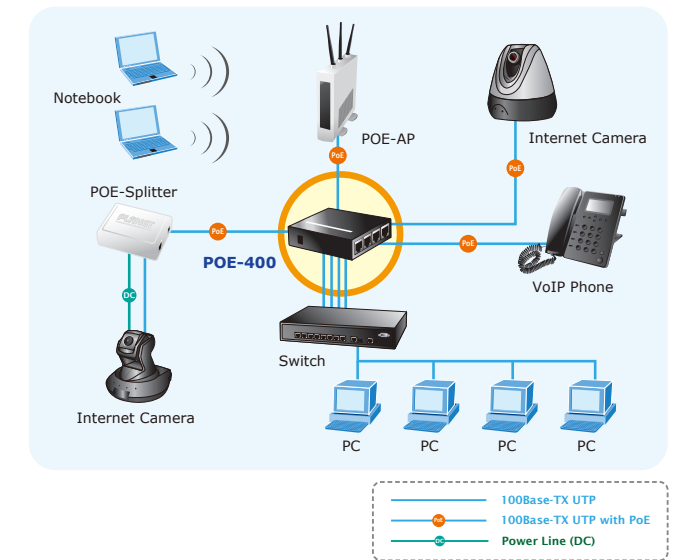
Figure 1: Connection architecture over POE-400
