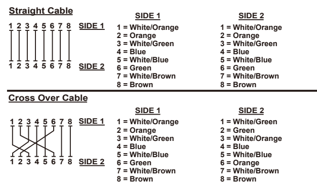
Figure A-1: Straight-Through and Crossover Cable
